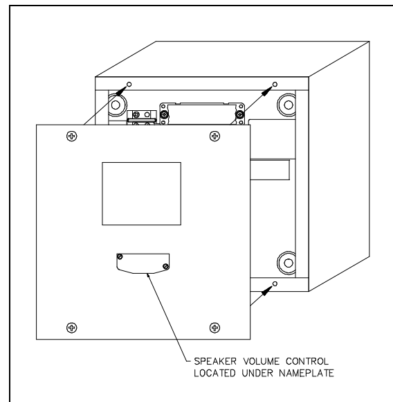
Figure 1. Model 751-001 Speaker Amplifier (shown with an indoor enclosure)
